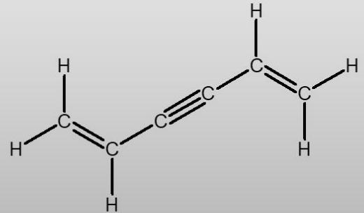
Divinylacetylen
